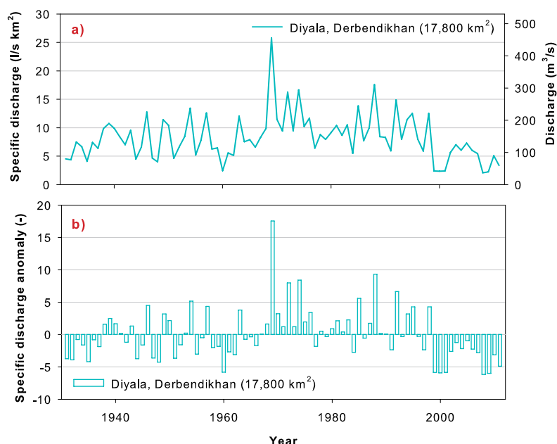
Figure 10. a) Mean annual discharge and b) discharge anomaly time series of the Diyala (1930-2011)
