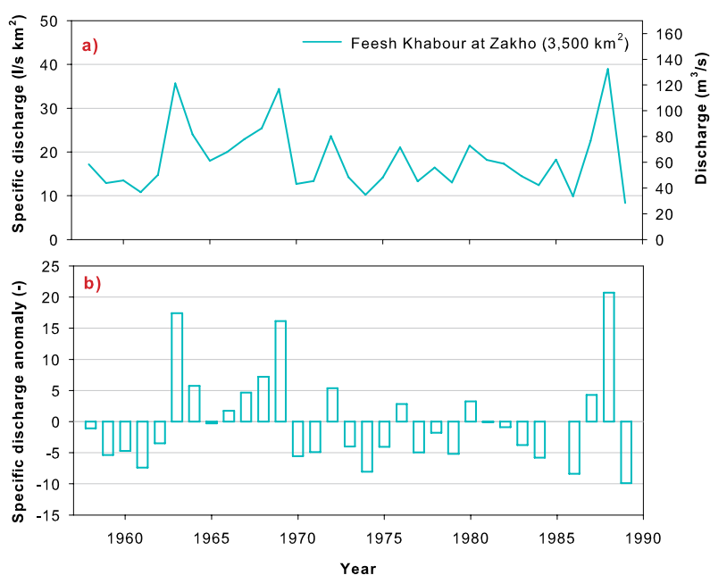
Figure 3. a) Mean annual discharge and b) discharge anomaly time series of the Feesh Khabour (1958-1989)
