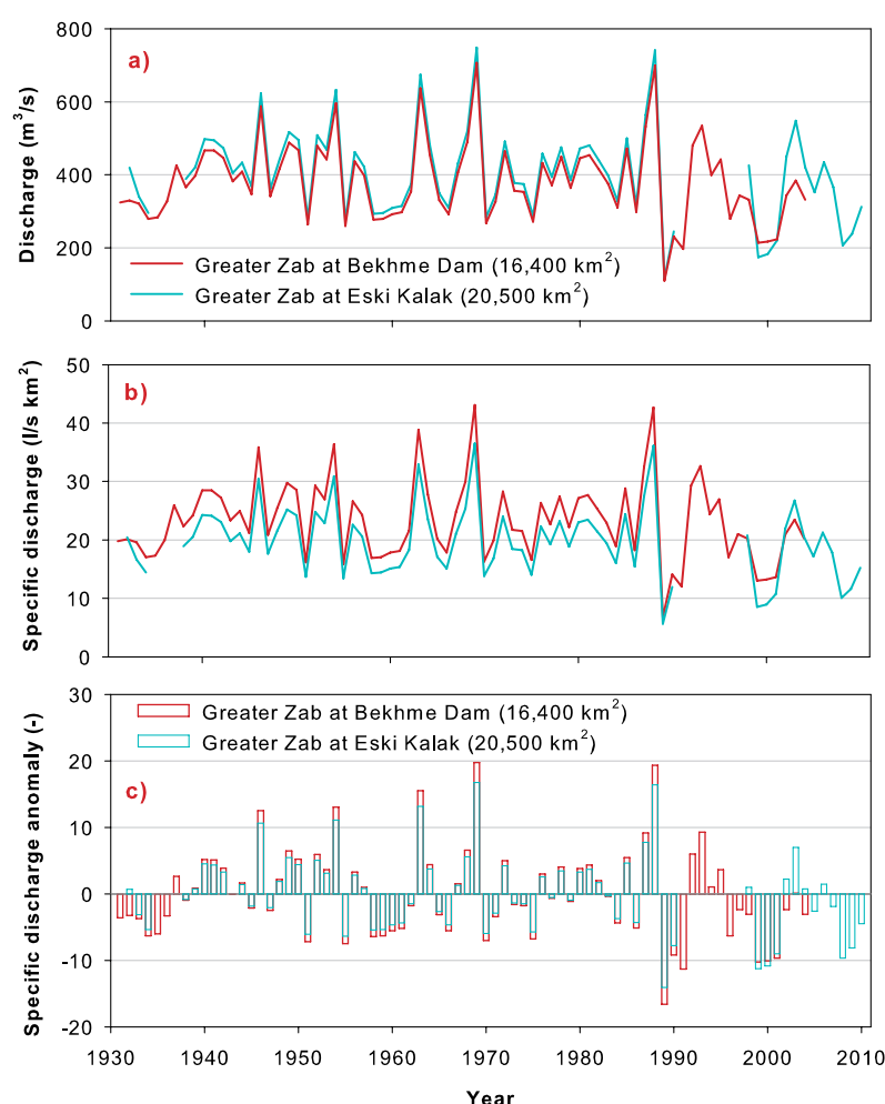
Figure 6. a) Mean annual discharge, b) specific mean annual discharge and c) discharge anomaly time series of the Greater Zab (1930-2011)
