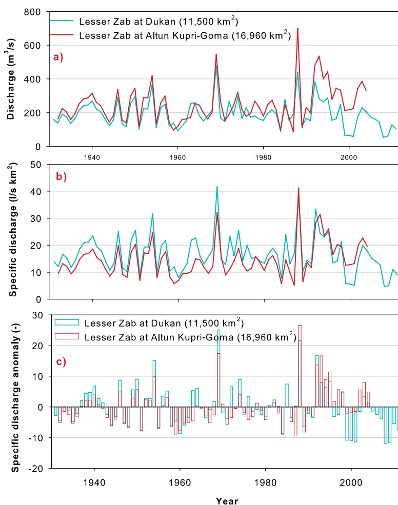
Figure 8. a) Mean annual discharge, b) specific mean annual discharge and c) discharge anomaly time series of the Lesser Zab (1930-2011)
